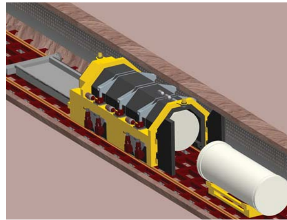
This cutaway of an emplacement tunnel shows the TEV placing a waste package in its designated spot.
