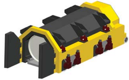
An electric transporter called a Transport and Emplacement Vehicle (TEV) will move into the waste handling facility to transport the waste package to the emplacement tunnels.
