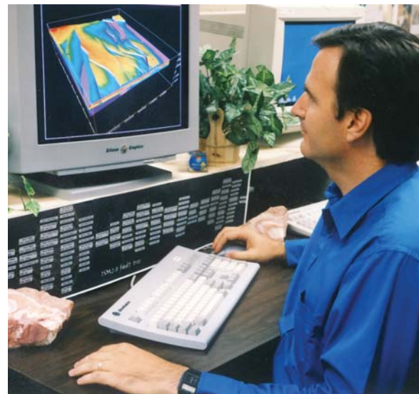
Scientists use both natural and man-made analogues to increase their confidence.
